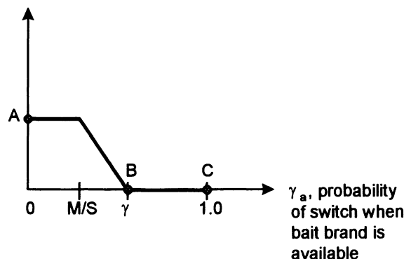
Probability of Stock Outage, \alpha
